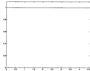
\alpha_2^2 as a function of \tau
