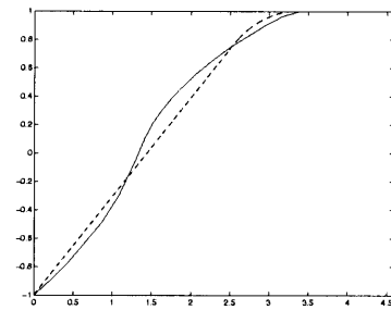
\alpha_2^1 as a function of \tau
