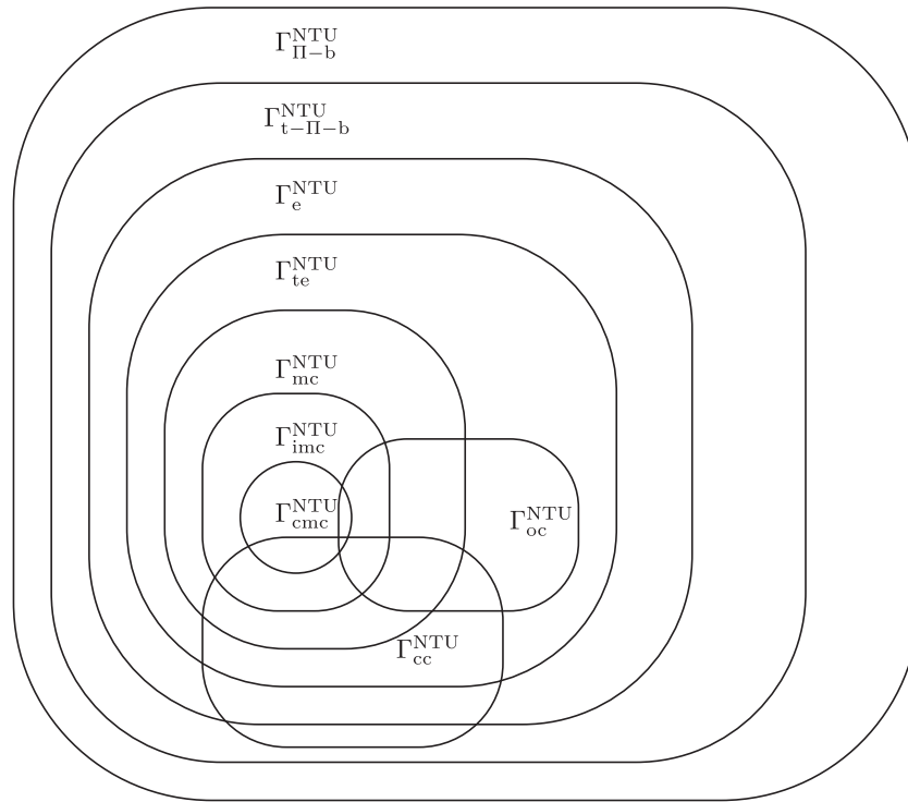
Fig. 1. Subsets of II-balanced games.
